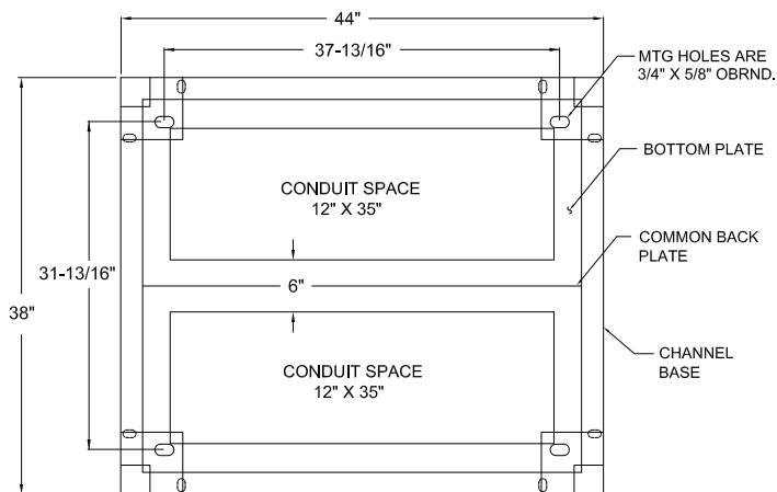
BOTTOM VIEW (SHOWING AVAILABLE CONDUIT SPACE)
