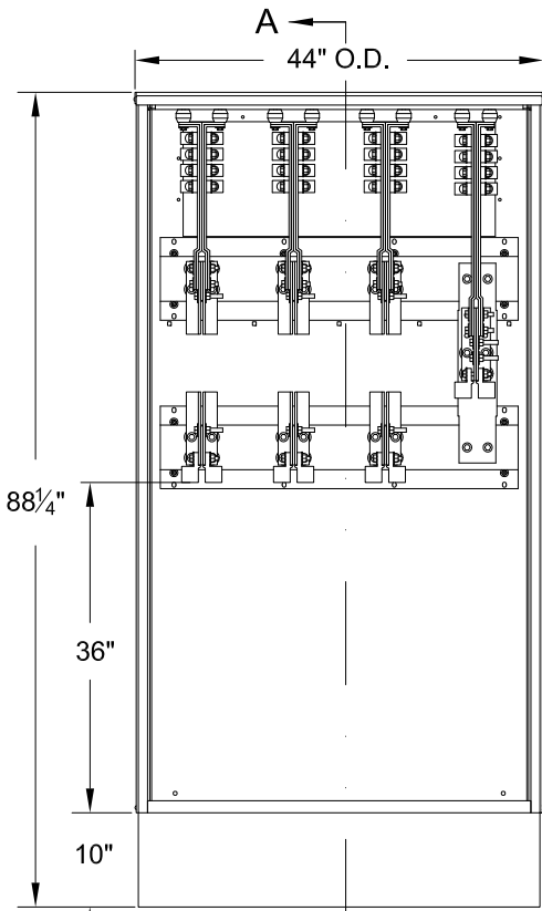
METERING TRANSFORMER COMPARTMENT (COVER REMOVED)
